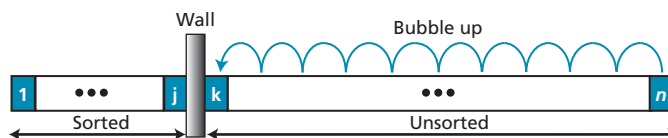
Figure 8.14 Bubble sort
