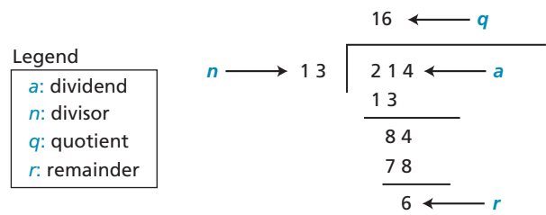
Figure G.1 Integer division
