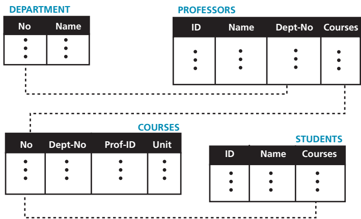
Figure 15.5 An example of the relational model representing a university
