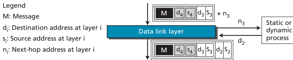
Figure 6.16 Addresses at the data link layer
