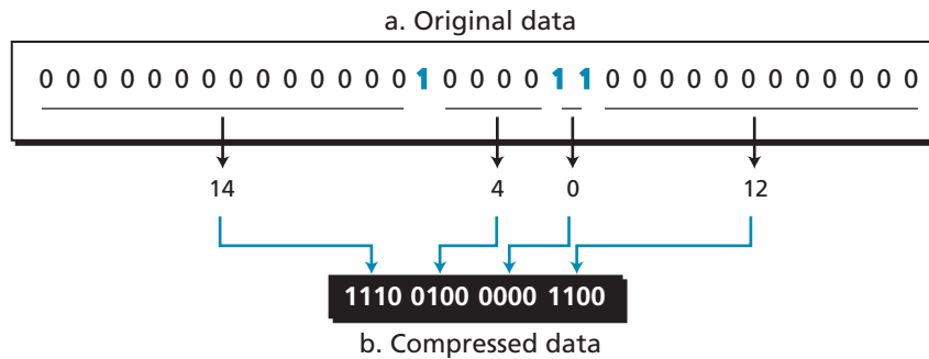
Figure 16.3 Run-length encoding for two symbols
