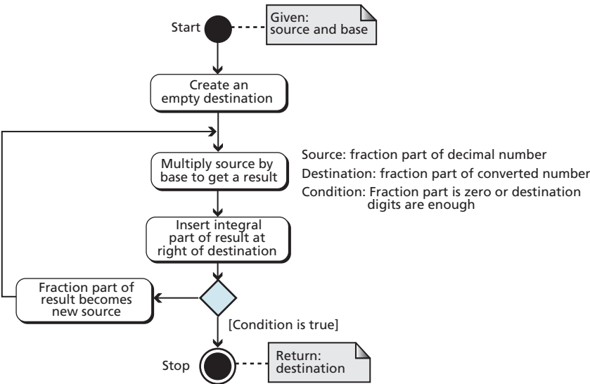
Figure 2.8 Algorithm to convert the fractional part of a decimal number to other bases
