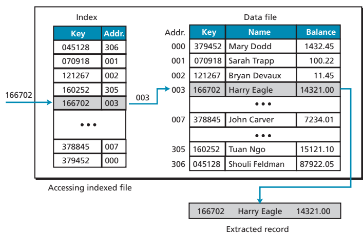
Figure 14.6 Logical view of an indexed file
