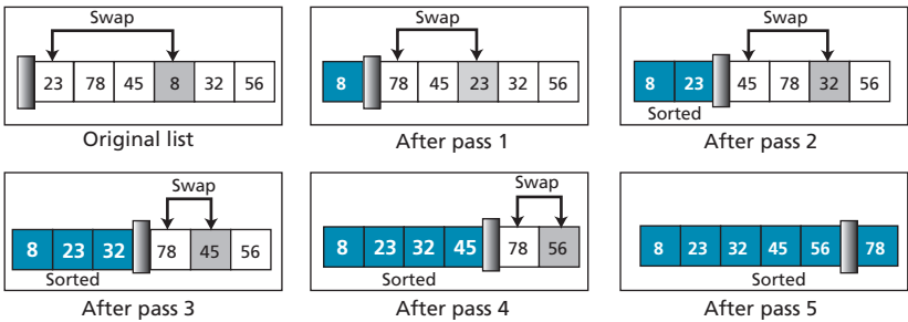
Figure 8.12 Example of selection sort
