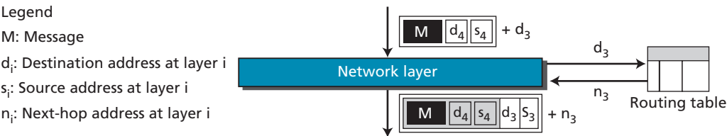
Figure 6.13 Addresses at the network layer
