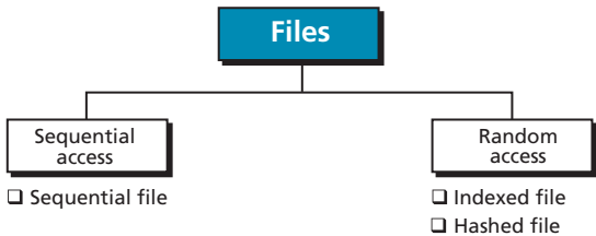
Figure 14.1 A taxonomy of file structures
