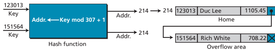
Figure 14.12 Linked list resolution
