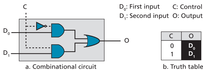
Figure E.15 Multiplexer
