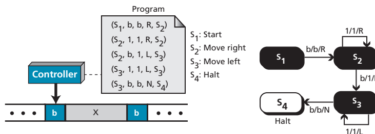
Figure 18.6 The Turing machine for the incr (X) statement
