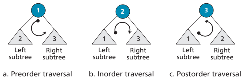
Figure 13.24 Depth-first traversal of a binary tree
