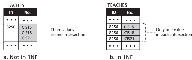
Figure 15.19 An example of 1NF
