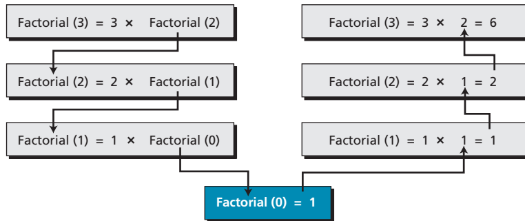
Figure 8.23 Tracing the recursive solution to the factorial problem
