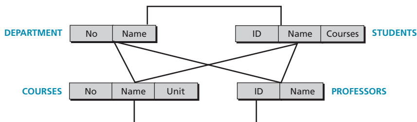
Figure 15.4 An example of the network model representing a university
