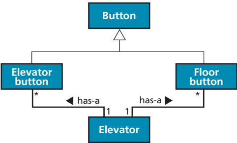
Figure 11.7 An example of a class diagram
