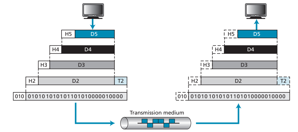
Figure 6.19 An exchange using the TCP/IP model
