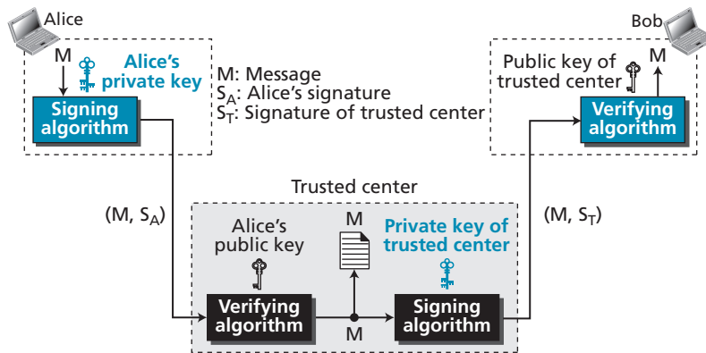
Figure 17.13 Nonrepudiation using digital signatures
