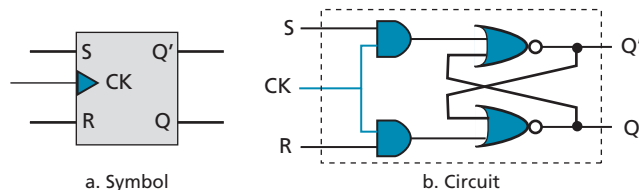
Figure E.22 Circuit of clocked SR flip-flop
