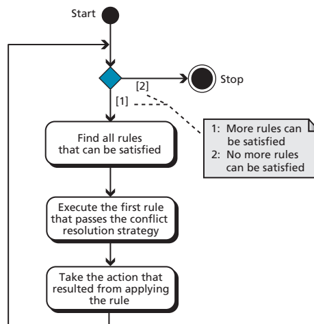
Figure 20.5 Flow diagram for forward chaining
