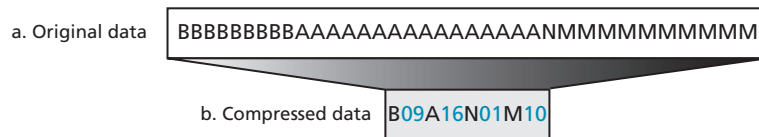
Figure 16.2 Run-length encoding example
