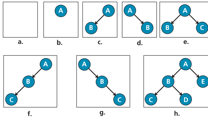
Figure 13.23 Examples of binary trees
