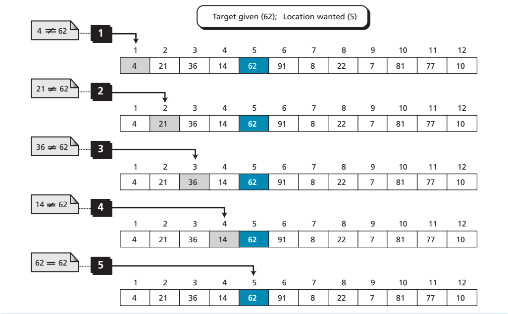
Figure 8.18 An example of a sequential search
