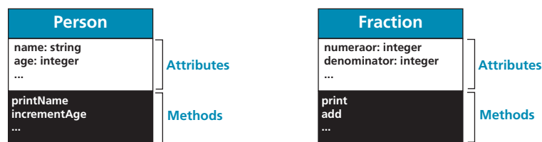
Figure B.5 Attributes and methods added to the class symbols
