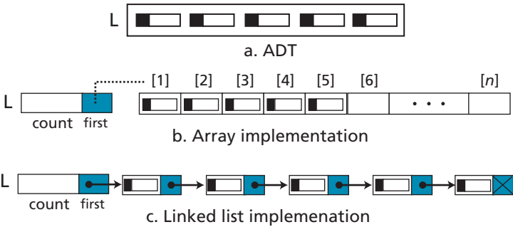
Figure 13.19 General linear list implementation
