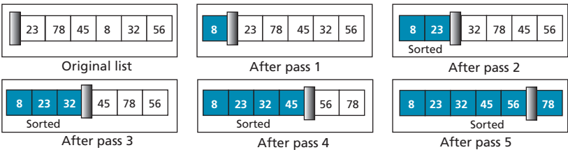
Figure 8.15 Example of bubble sort
