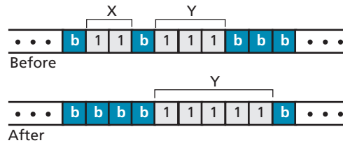
Figure 18.11 Configuration of the tapes for Example 18.4
