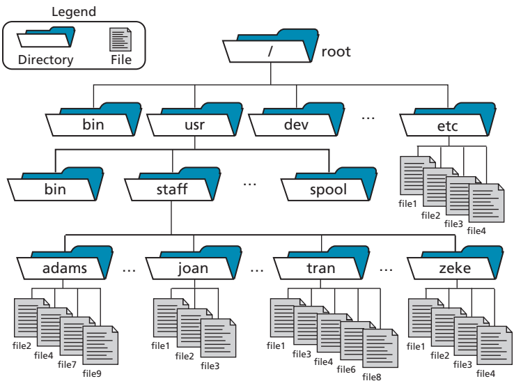
Figure 14.14 An example of directory system in UNIX
