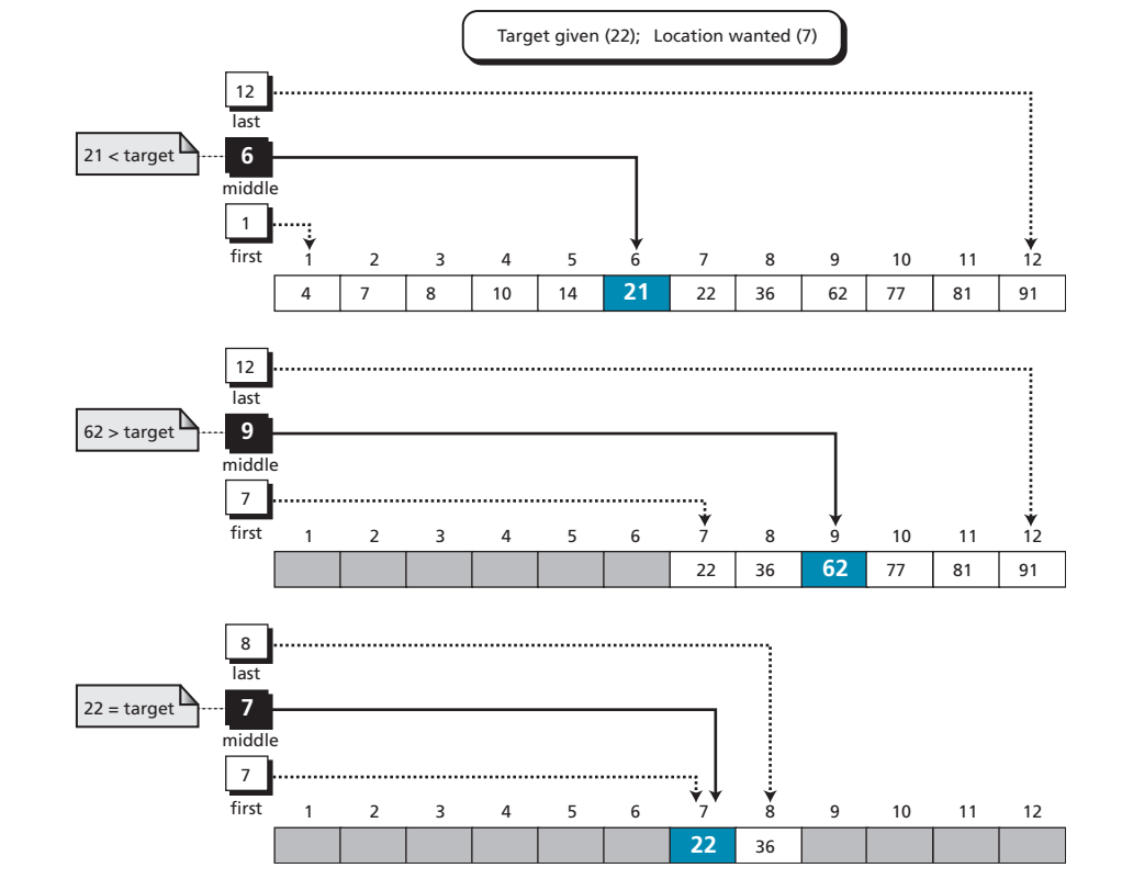
Figure 8.19 Example of a binary search
