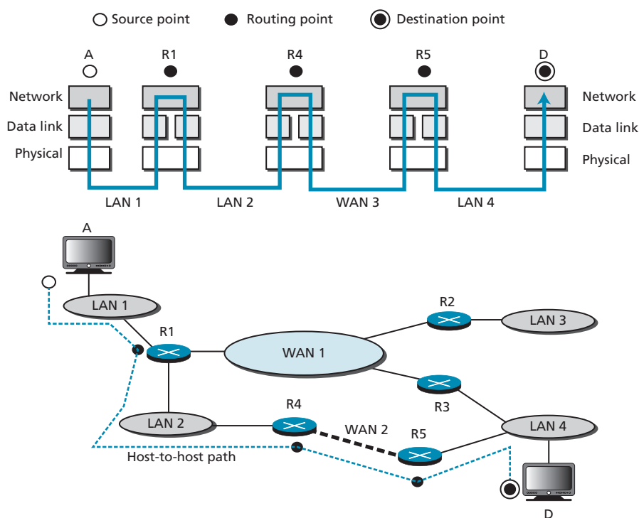
Figure 6.14 Routing at the network layer
