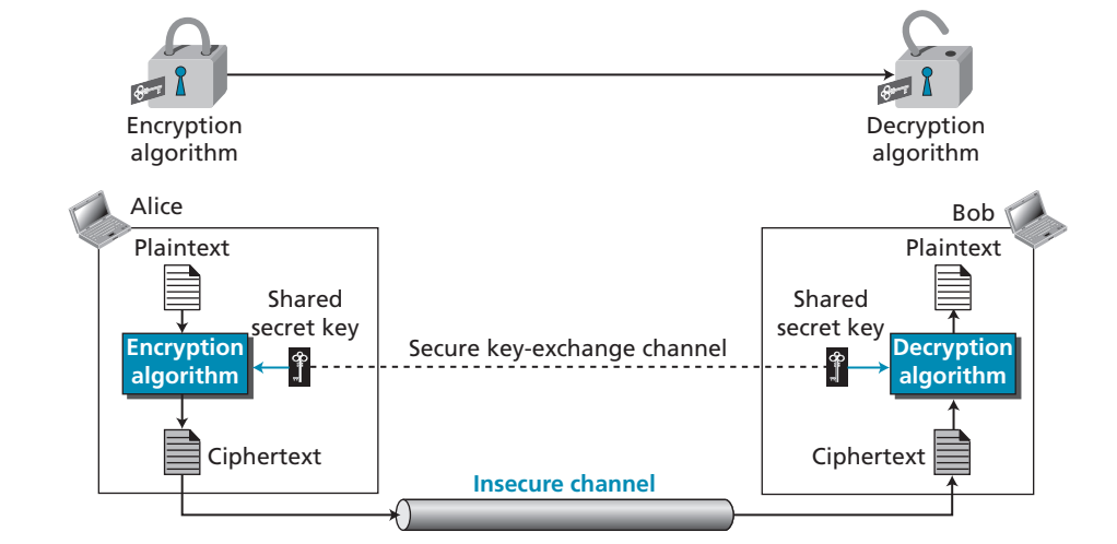
Figure 17.4 The general idea of symmetric-key cryptography
