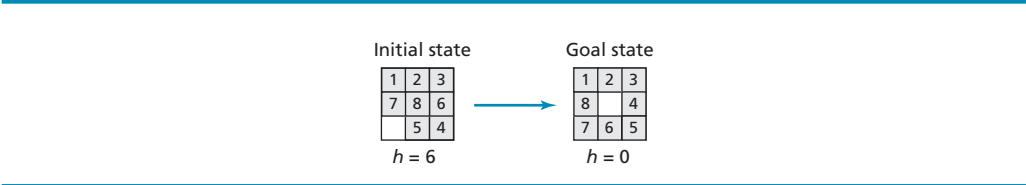
Figure 20.19 Initial and goal states for heuristic search
