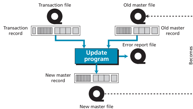
Figure 14.3 Updating a sequential file
