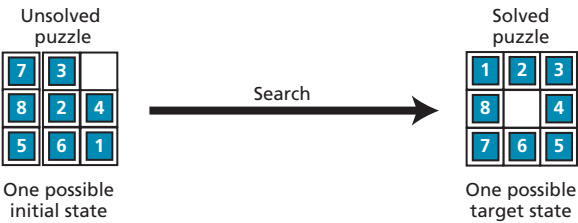
Figure 20.14 The initial and possible states for Example 20.6
