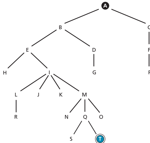
Figure 20.16 The tree for the maze in Figure 20.15
