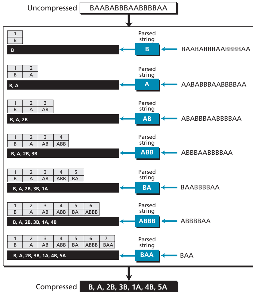
Figure 16.10 An example of Lempel Ziv encoding
