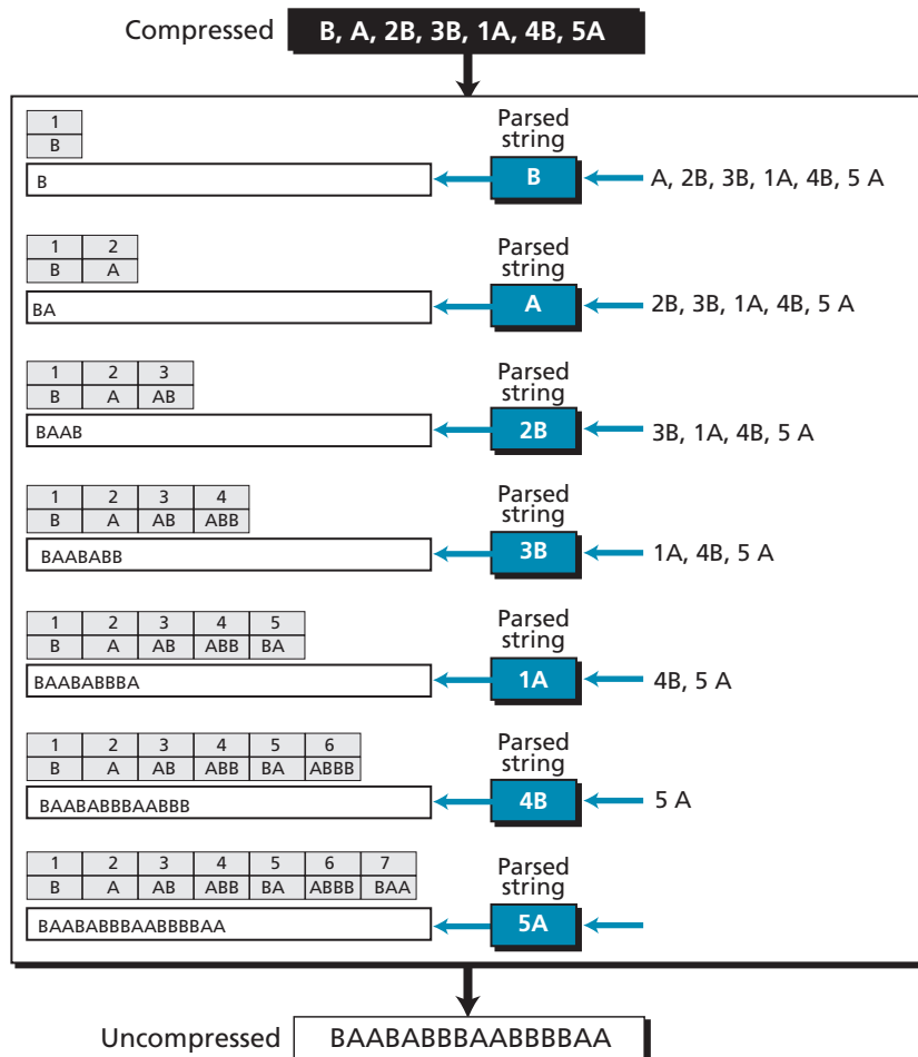
Figure 16.11 An example of Lempel Ziv decoding
