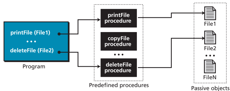
Figure 10.3 The concept of the procedural paradigm
