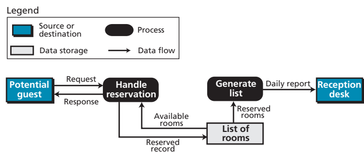
Figure 11.4 An example of a data flow diagram
