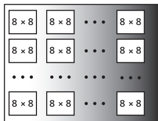
Figure 16.12 JPEG grayscale example, 640 \times 480 pixels
