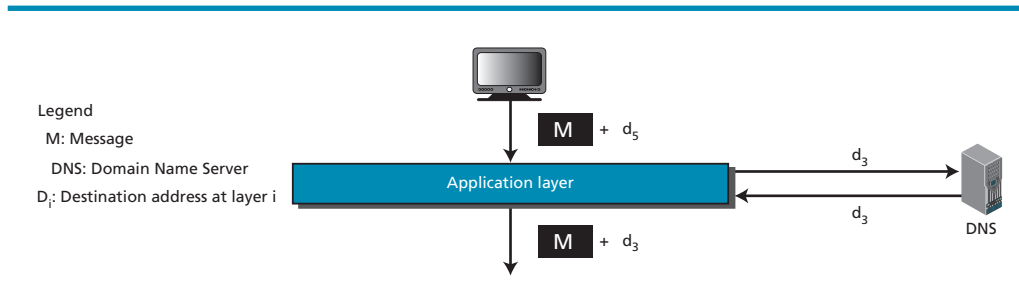
Figure 6.10 Addresses at the application layer
