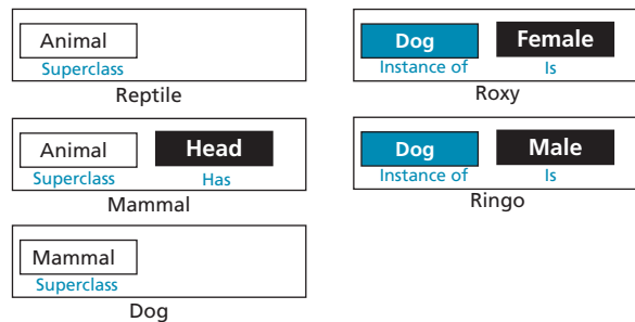
Figure 20.2 A set of frames representing semantic network
