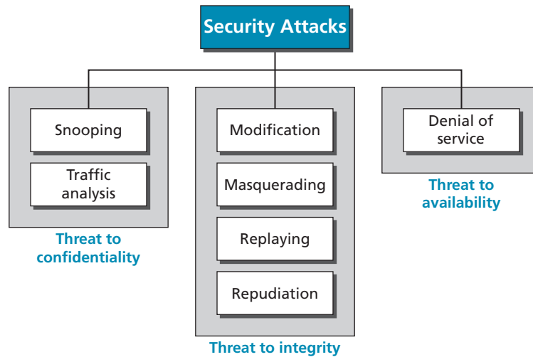
Figure 17.2 Taxonomy of attacks with relation to security goals
