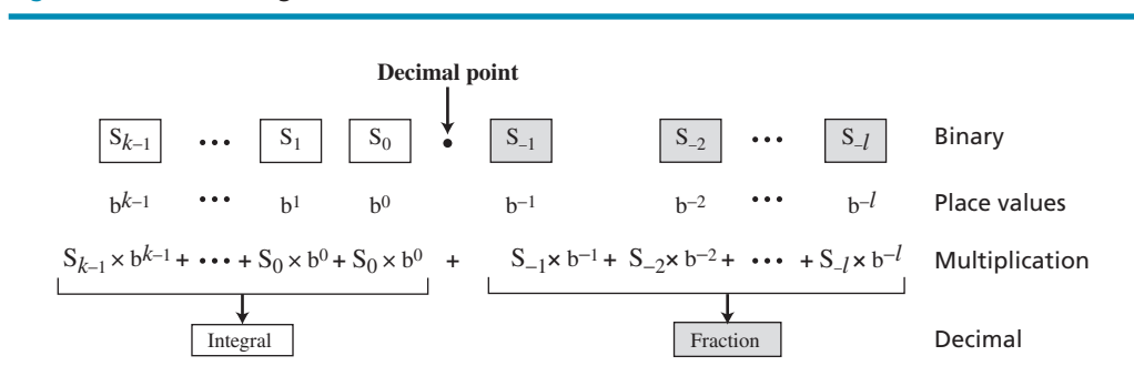
Figure 2.5 Converting other bases to decimal
