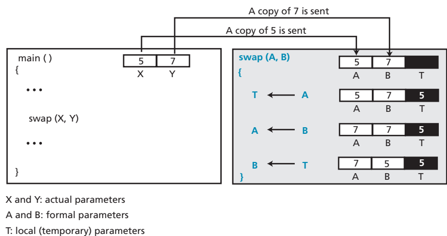
Figure 10.13 An example in which pass by value does not work
