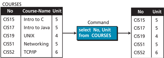
Figure 15.11 An example of a project operation
