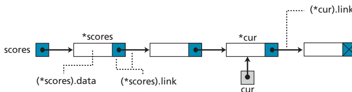
Figure 12.12 The name of a linked list versus the names of nodes
