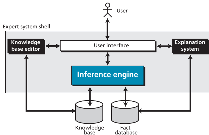
Figure 20.7 The architecture of an expert system
