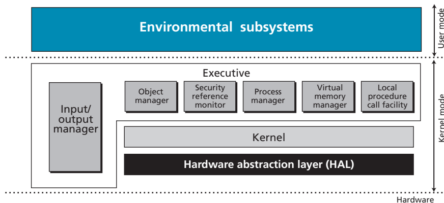
Figure 7.21 The architecture of Windows NT
