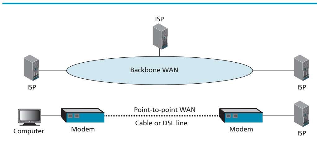
Figure 6.4 A point-to-point WAN and a backbone WAN
