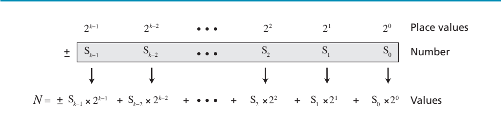
Figure 2.2 Place values in an integer in the binary system
