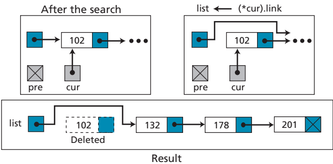
Figure 12.18 Deleting the first node of a linked list
