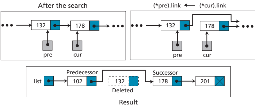
Figure 12.19 Deleting a node at the middle or end of a linked list
