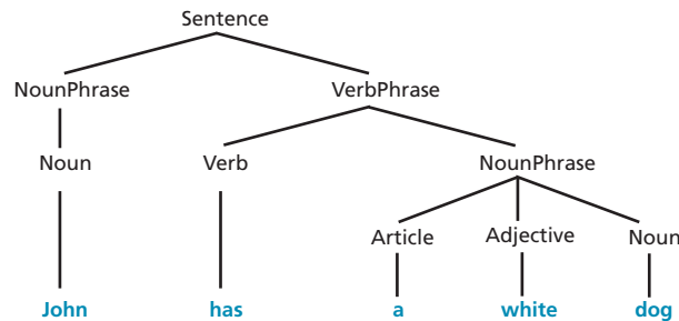
Figure 20.12 Parsing a sentence
