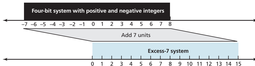
Figure 3.11 Shifting in Excess representation
