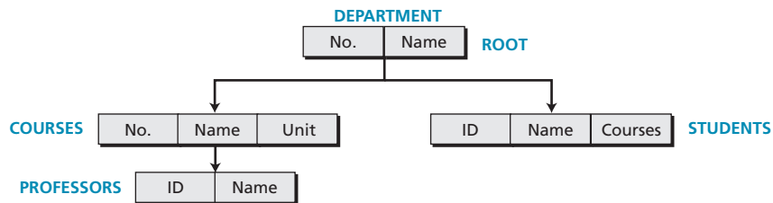
Figure 15.3 An example of the hierarchical model representing a university
