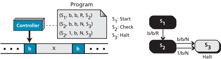
Figure 18.8 The Turing machine for the \text{decr}(X) statement
