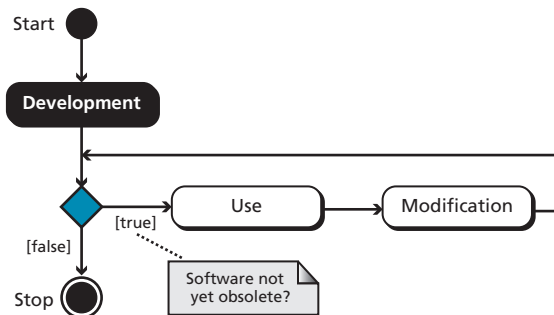
Figure 11.1 The software life cycle
