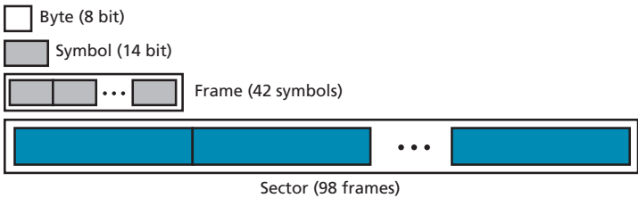
Figure 5.9 CD-ROM format
