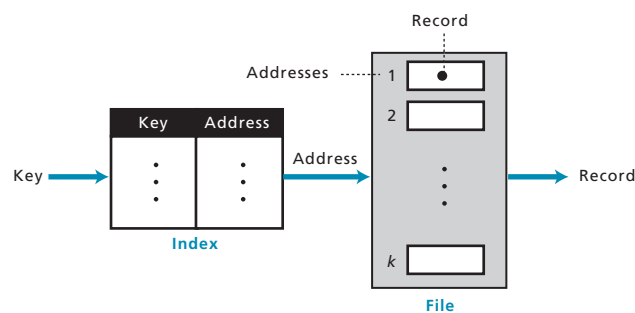
Figure 14.5 Mapping in an indexed file
