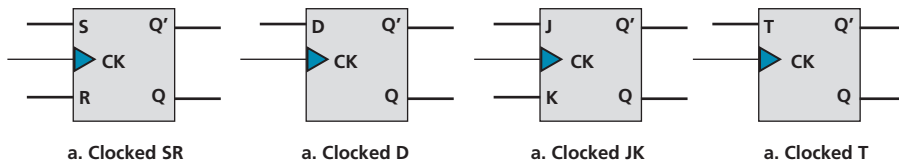
Figure E.21 Clocked flip-flops
