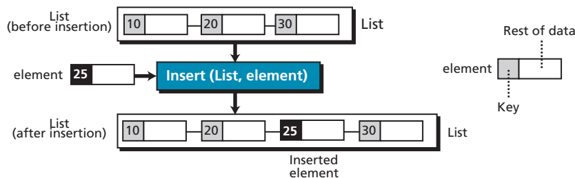
Figure 13.15 The insert operation
