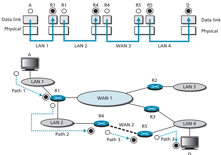
Figure 6.15 Communication at the data-link layer
