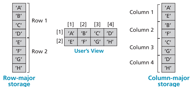
Figure 12.6 Memory layout of arrays
