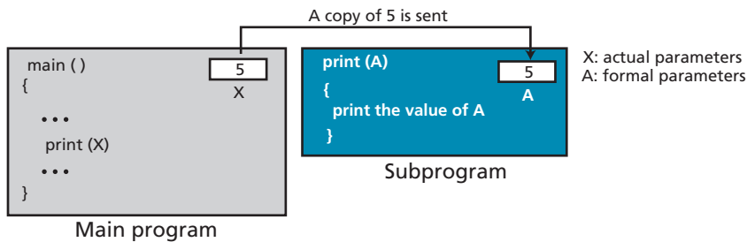
Figure 10.12 An example of pass by value
