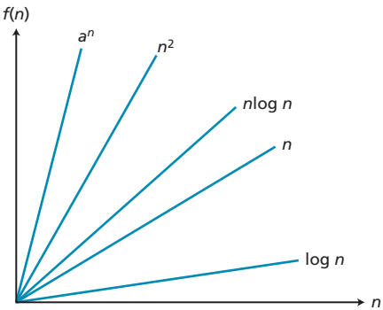
Figure 9.6 Relationship between common algorithms discussed in this chapter
