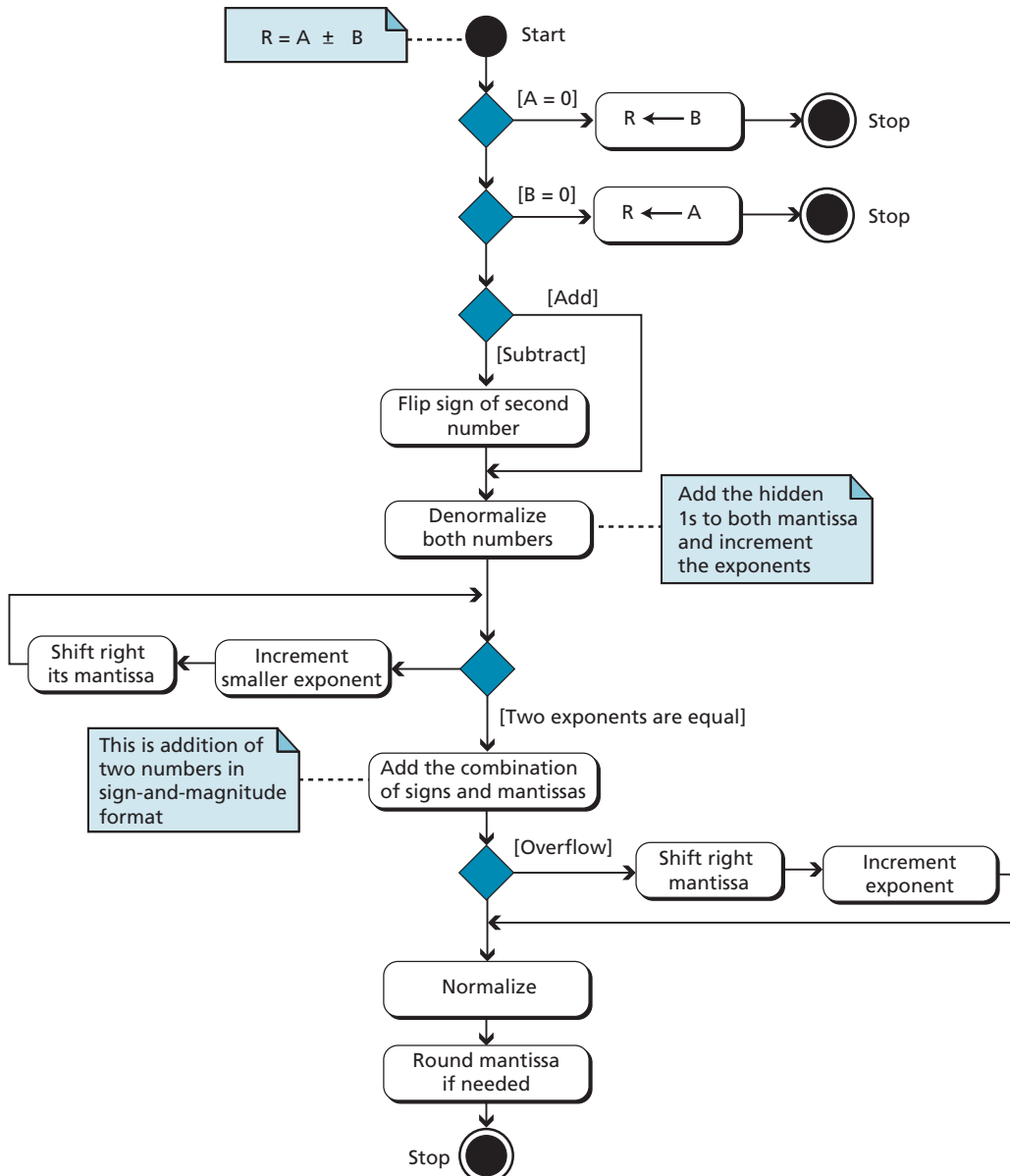
Figure 4.8 Addition and subtraction of reals in floating-point format
