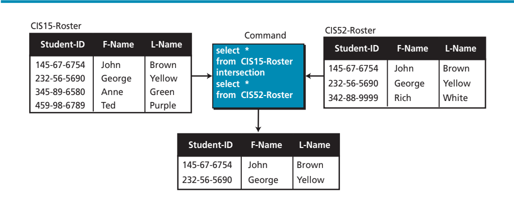
Figure 15.14 An example of an intersection operation
