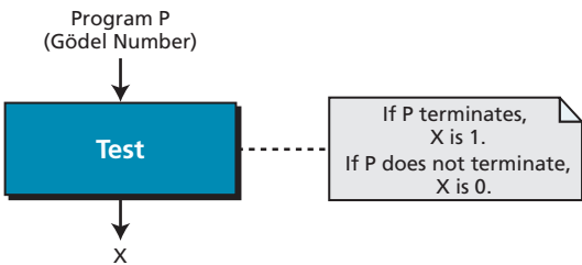
Figure 18.14 Step 1 in the proof
