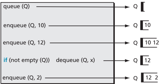
An algorithm segment
