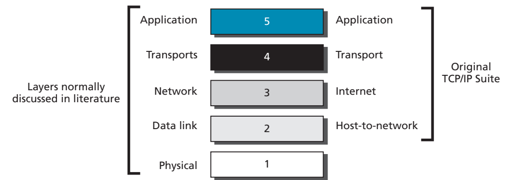
Figure 6.7 The TCP/IP protocol suite
