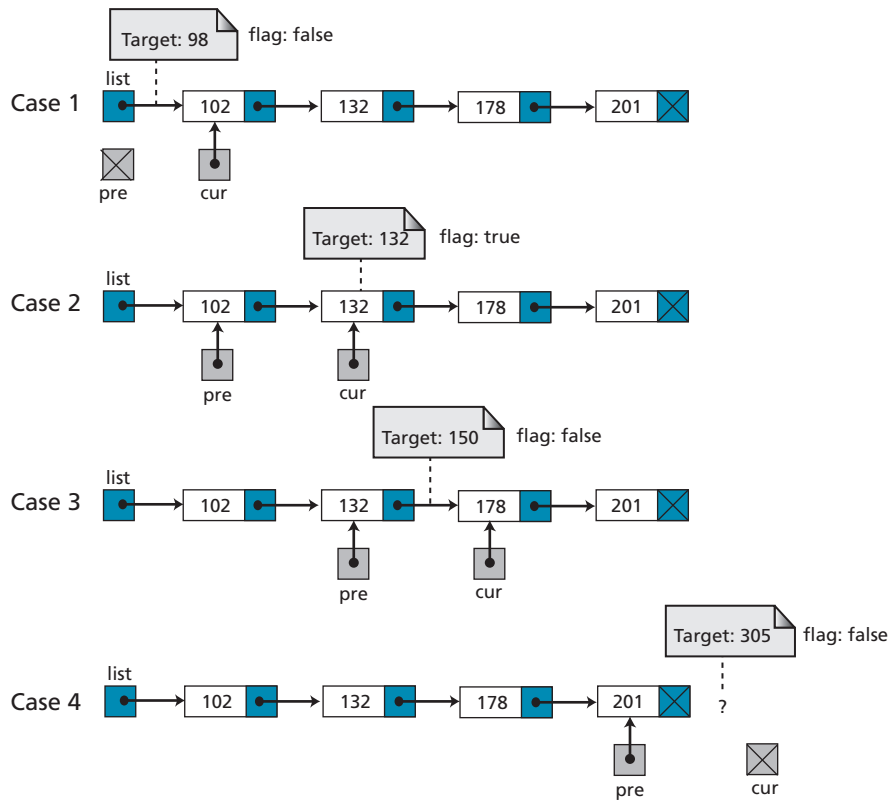
Figure 12.14 Values of pre and cur pointers in different cases
