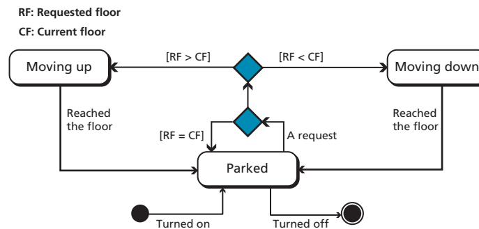
Figure 11.5 An example of a state diagram
