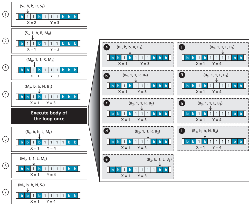
Figure 18.13b Second iteration in Example 18.4 (Continued)
