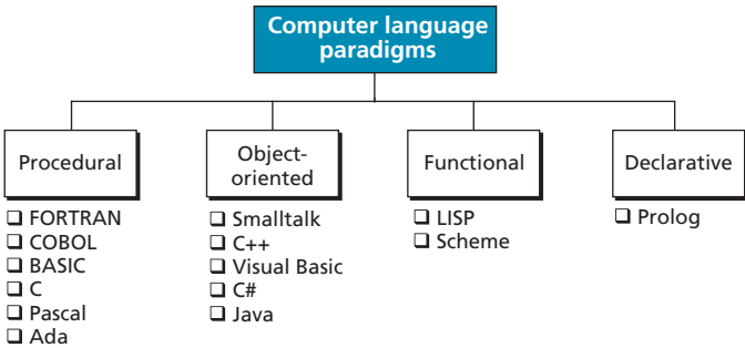
Figure 10.2 Categories of programming languages
