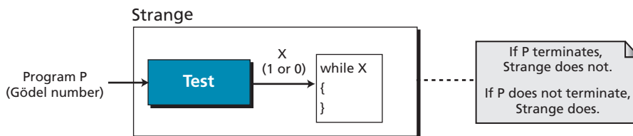
Figure 18.15 Step 2 in the proof
