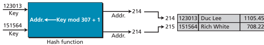
Figure 14.11 Open addressing resolution
