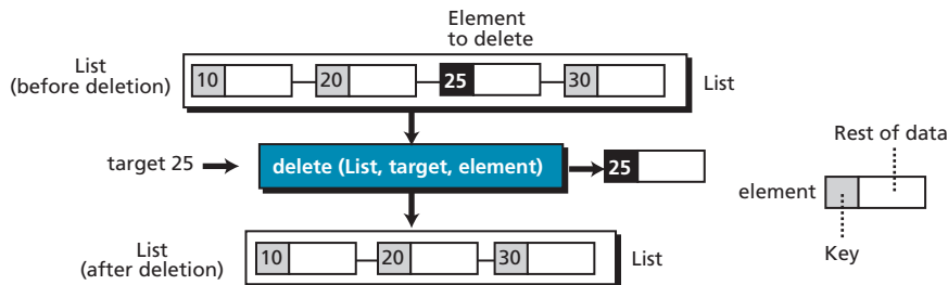
Figure 13.16 The delete operation
