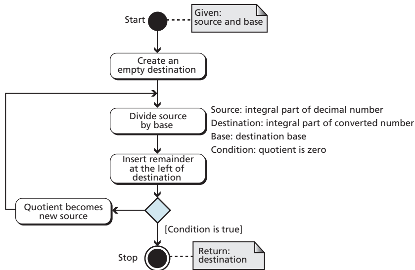
Figure 2.6 Converting the integral part of a decimal number to other systems
