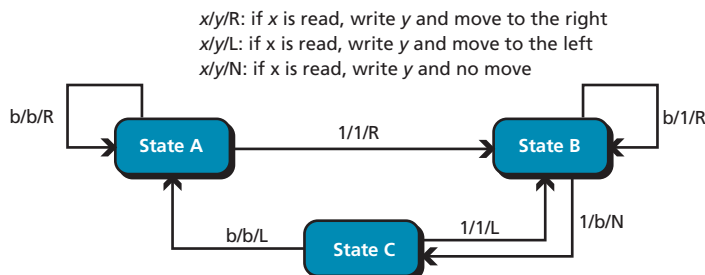
Figure 18.4 Transition state diagram for the Turing machine
