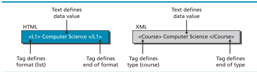
Figure 6.31 Comparing HTML and XML
