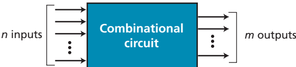
Figure E.13 A combinational circuit
