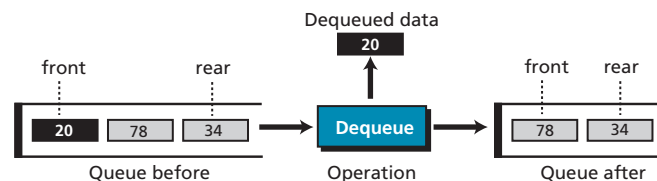
Figure 13.11 The dequeue operation
