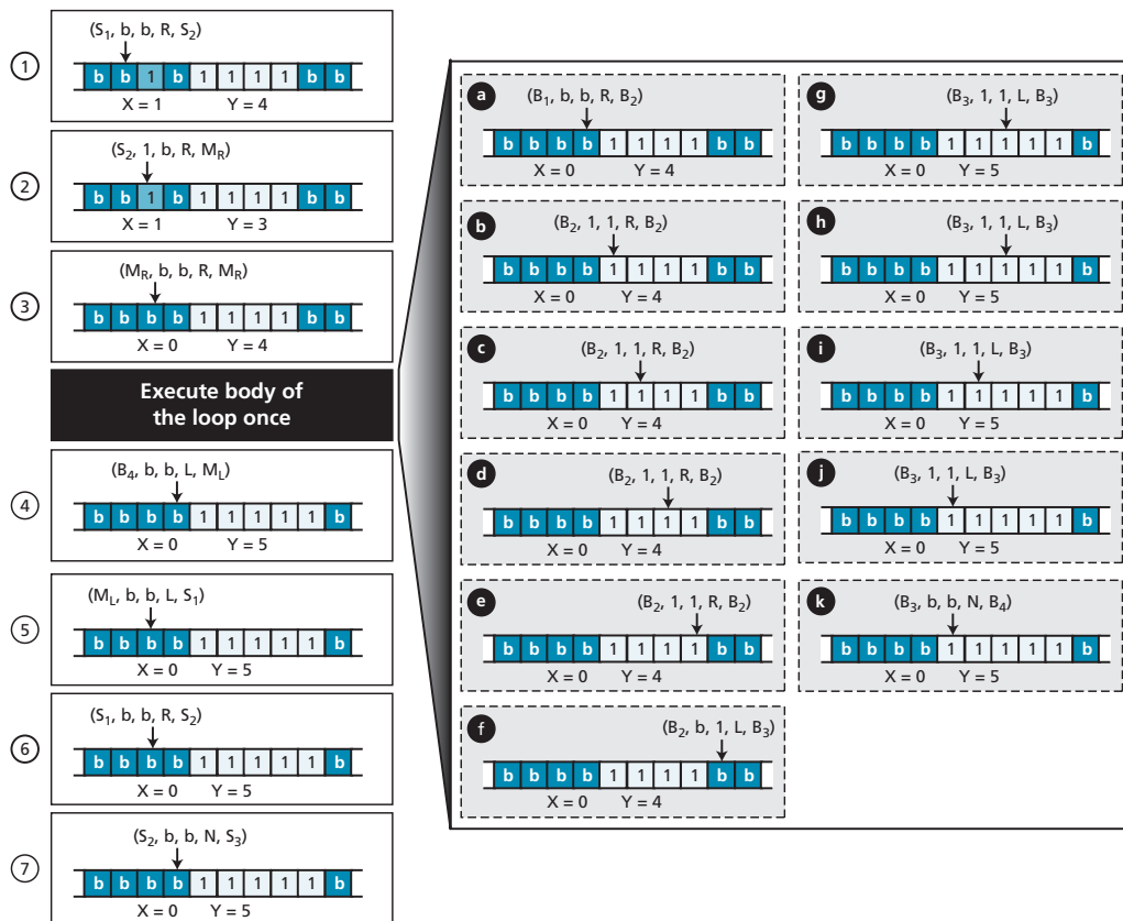
Figure 18.13a Second iteration in Example 18.4
