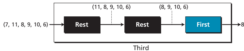
Figure 10.8 Extracting the third element of a list
