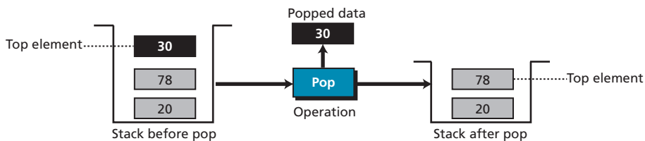
Figure 13.5 Pop operation
