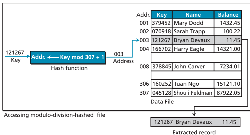
Figure 14.9 Modulo division
