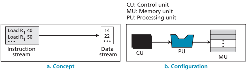
Figure 5.26 SISD organization
