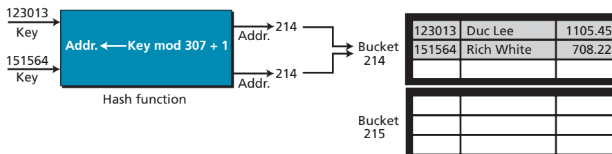
Figure 14.13 Bucket hashing resolution
