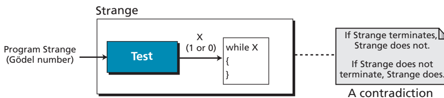
Figure 18.16 Step 3 in the proof
