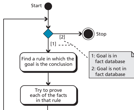
Figure 20.6 Flow diagram for backward chaining
