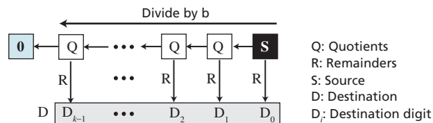
Figure 2.7 Converting the integral part
