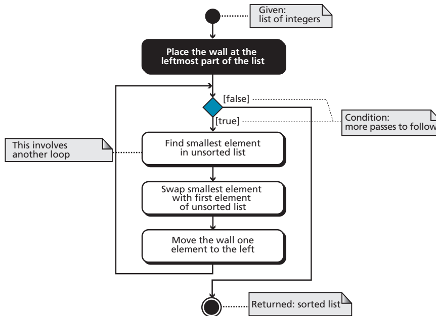
Figure 8.13 Selection sort algorithm
