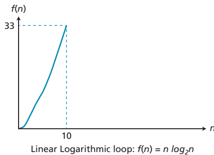
Figure 9.3 Linear logarithmic algorithm
