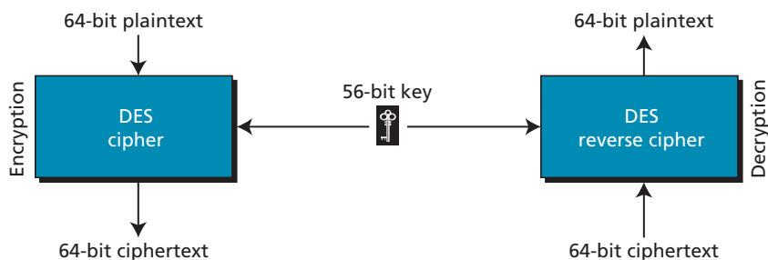
Figure 17.5 Encryption and decryption with DES
