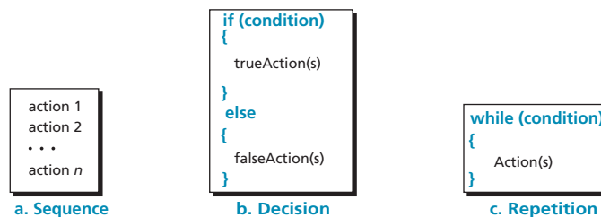
Figure 8.8 Pseudocode for three constructs
