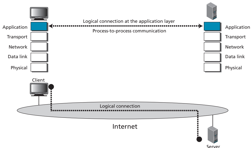
Figure 6.9 Communication at the application layer
