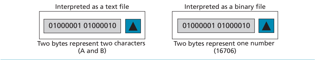
Figure 14.15 Text and binary interpretations of a file
