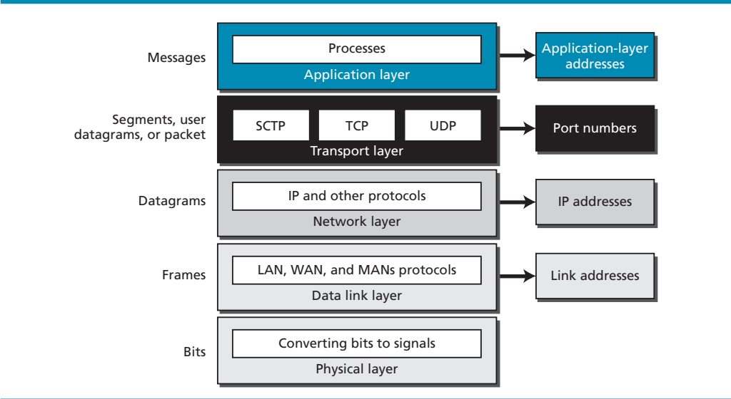
Figure 6.18 Four level of addressing in the internet
