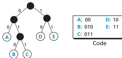
Figure 16.5 Final tree and code
