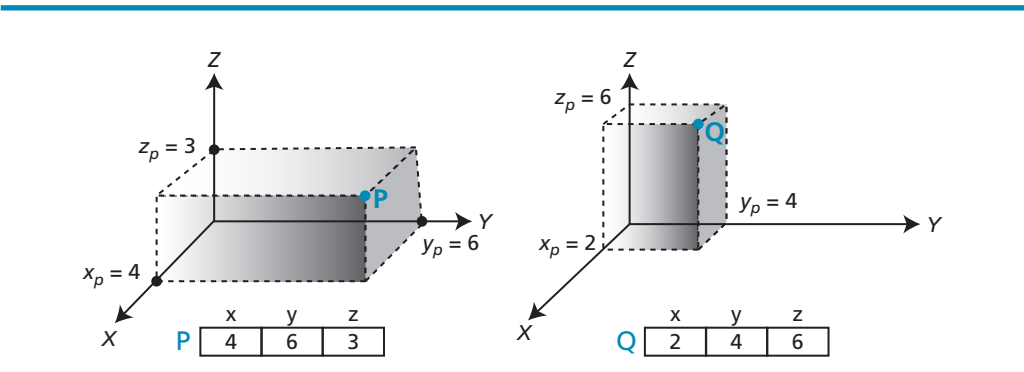
Figure 19.1 Representation of independent points in space
