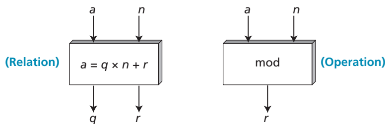
Figure G.2 Division relation versus modulo operator
