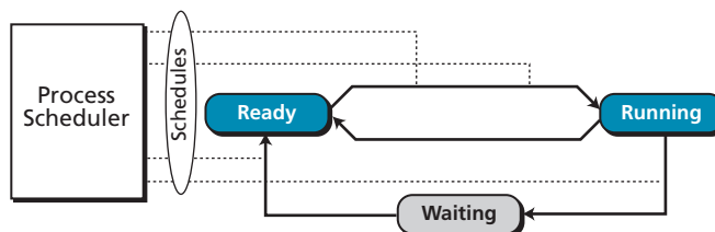
Figure 7.14 Process scheduler
