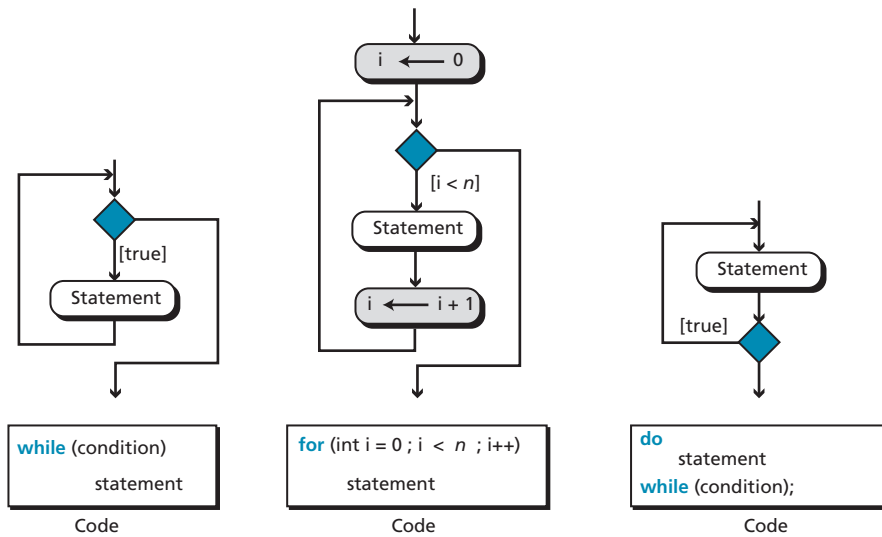
Figure 10.10 Three types of repetition
