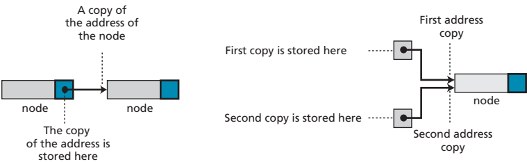
Figure 12.10 The concept of copying and storing pointers
