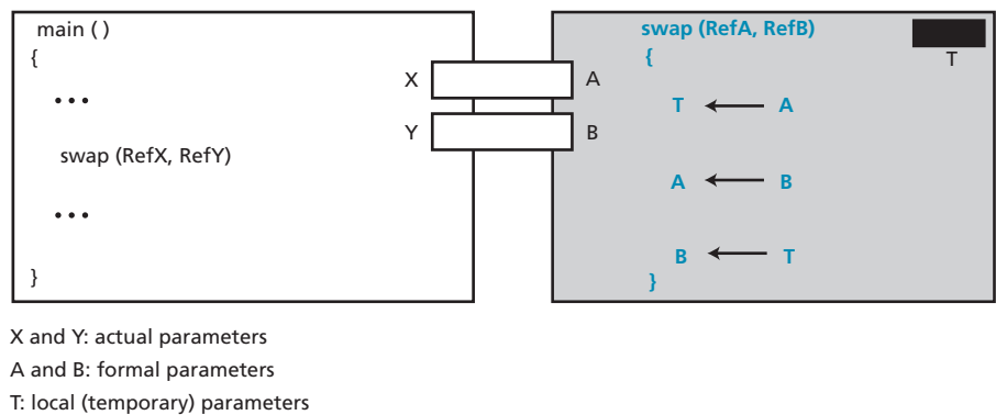
Figure 10.14 An example of pass by reference
