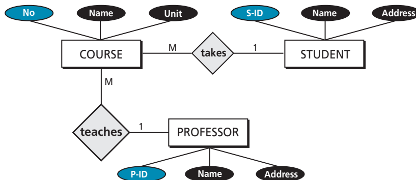
Figure 15.16 Entities, attributes, and relationships in an E-R diagram
