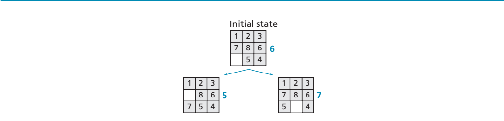
Figure 20.20 The heuristic values for the first step
