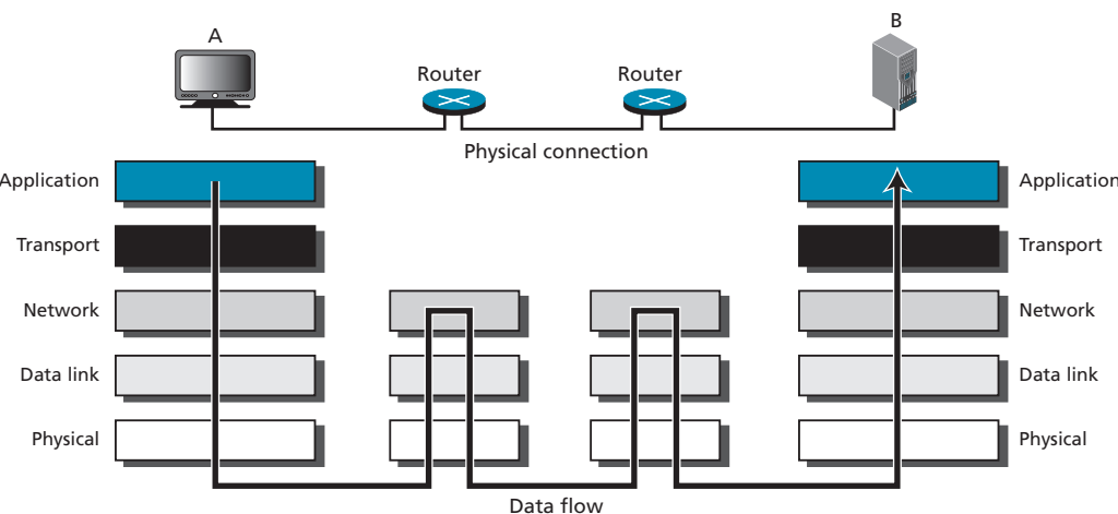
Figure 6.8 The interaction between layers in the TCP/IP protocol suite
