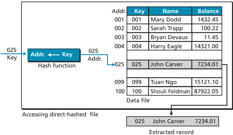
Figure 14.8 Direct hashing
