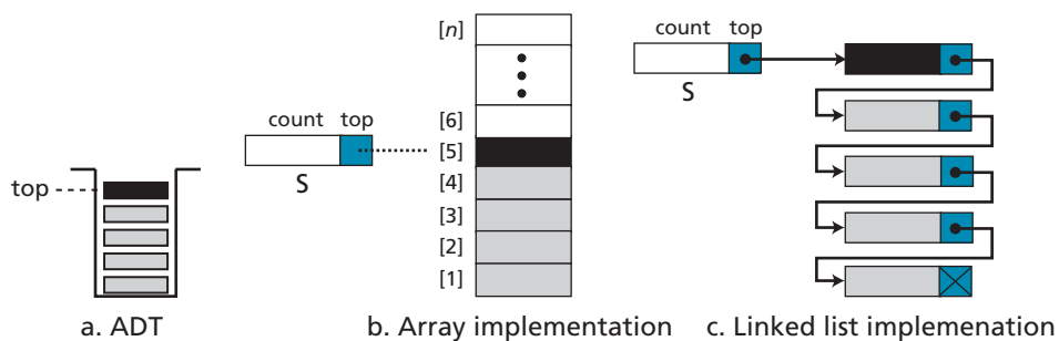
Figure 13.7 Stack implementations
