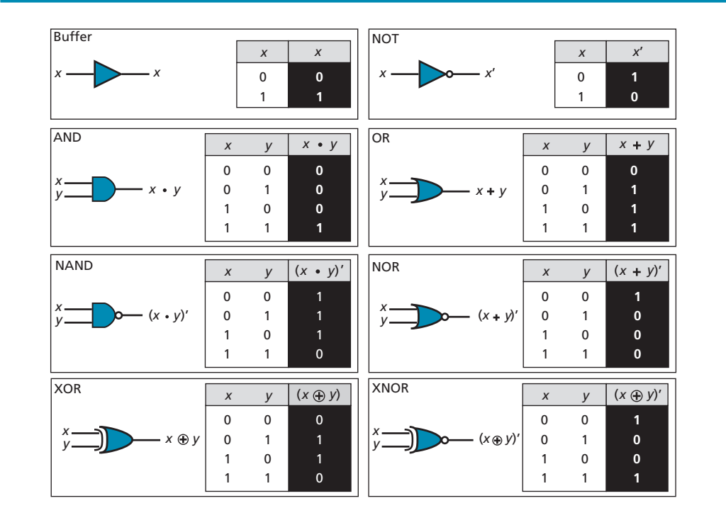
Figure E.1 Symbols and truth table for common gates
