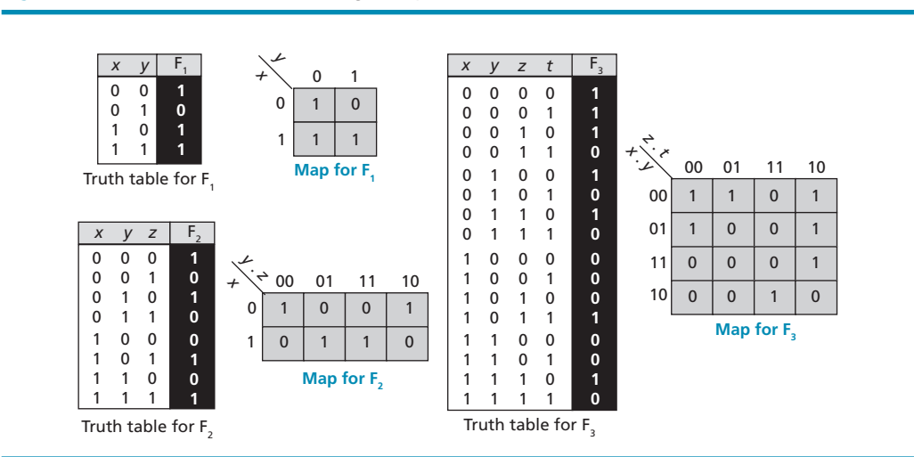
Figure E.8 Construction of Karnaugh maps
