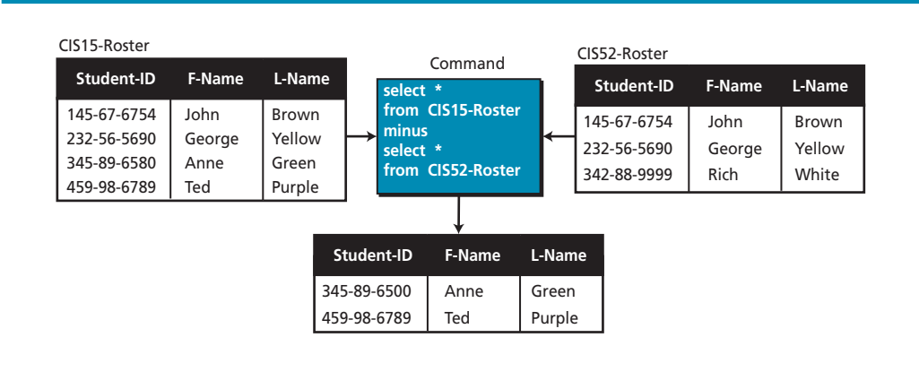
Figure 15.15 An example of a difference operation
