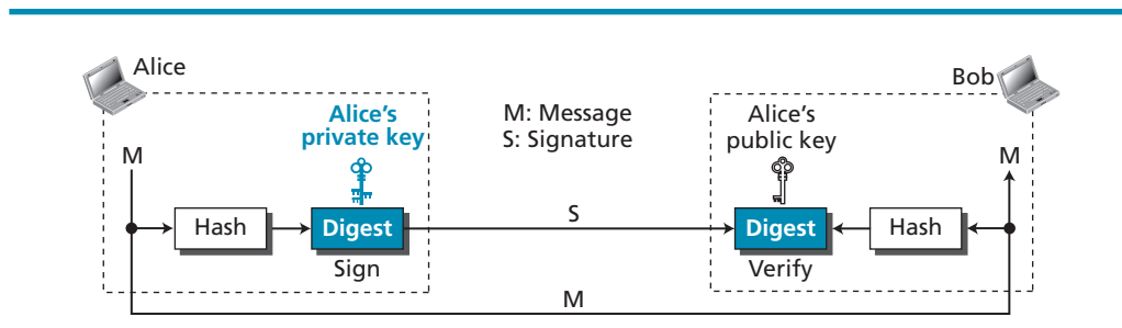
Figure 17.12 Signing the digest
