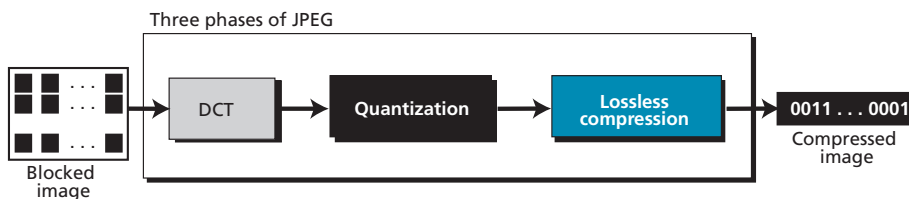
Figure 16.13 The JPEG compression process
