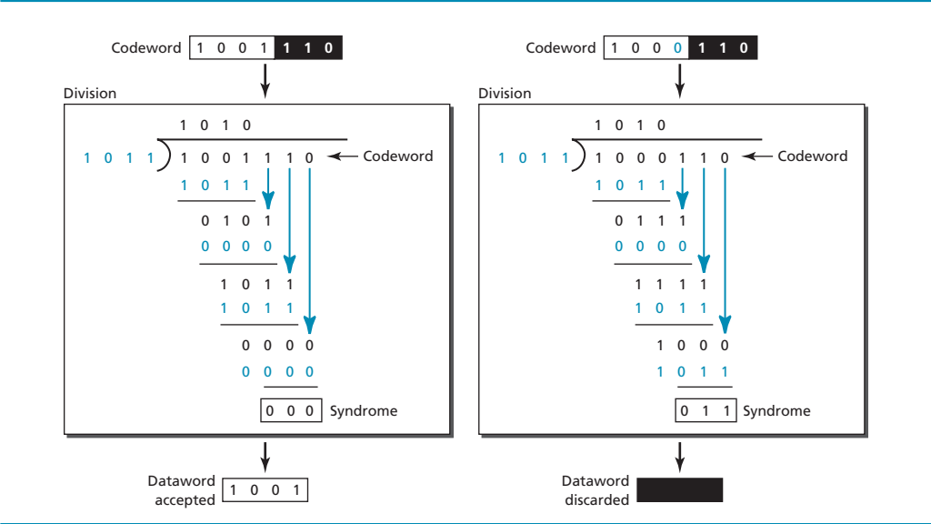
Figure H.9 Division in the CRC decoder for two cases
