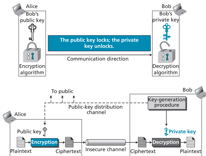
Figure 17.7 The general idea behind asymmetric-key cryptography
