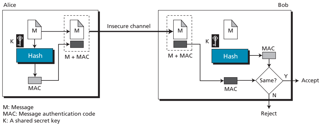
Figure 17.10 Message authentication code
