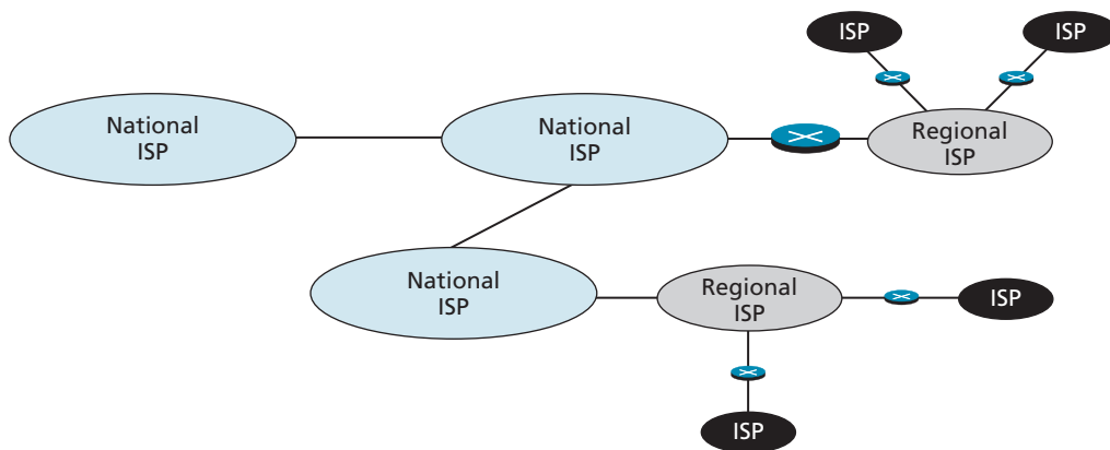
Figure 6.6 Hierarchical organization of the internet
