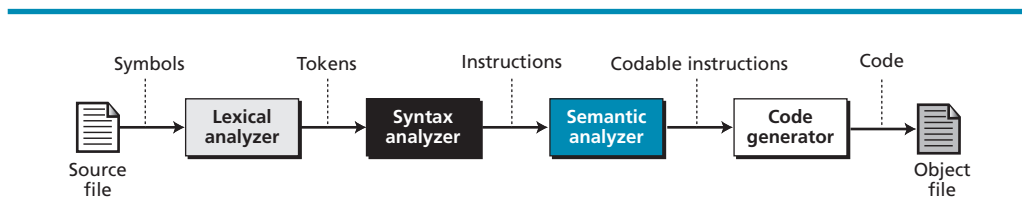
Figure 10.1 Source code translation process
