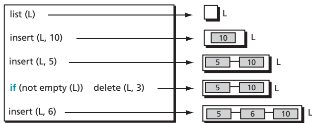
An algorithm segment
