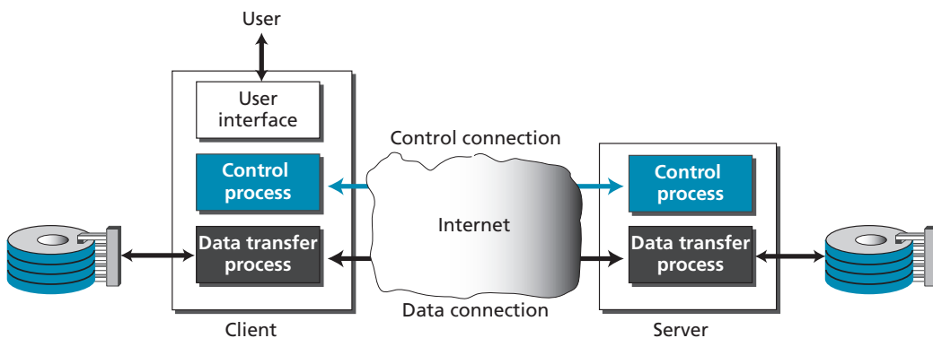
Figure 6.23 File Transfer Protocol (FTP)
