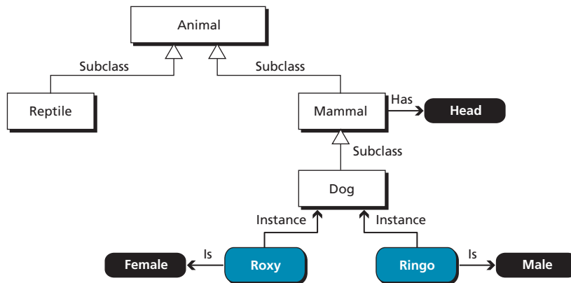
Figure 20.1 A simple semantic network
