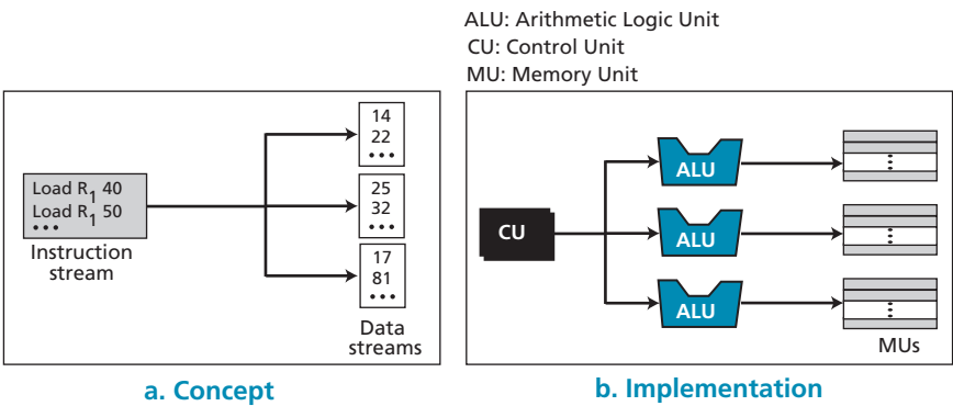
Figure 5.27 SIMD organization
